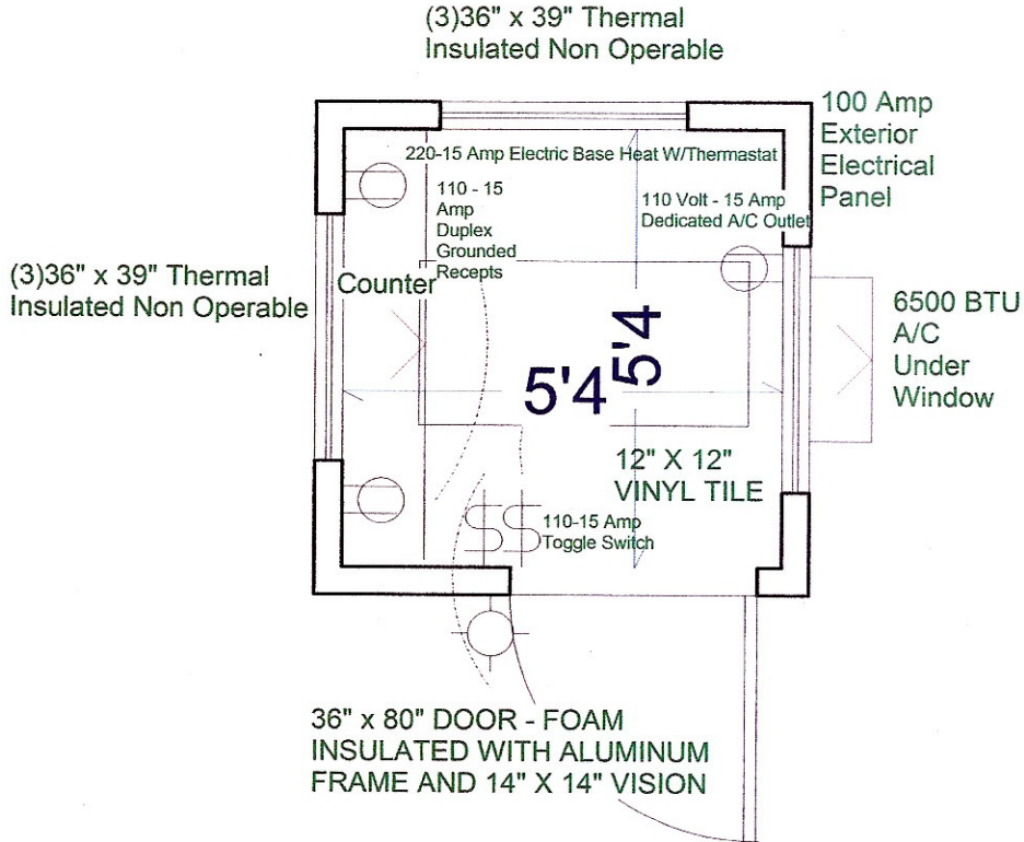
Operators Booth 6' x 6' Standard Guardhouse - Plan A
